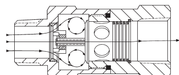
Check Valve In Closed Position
